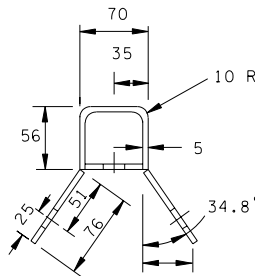
SECTION "G-G" SIDE VIEW
