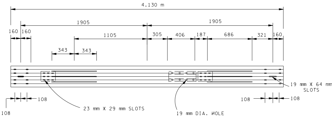
FIRST SECTION OF GUARDRAIL FOR TYPE 21 TERMINALS
