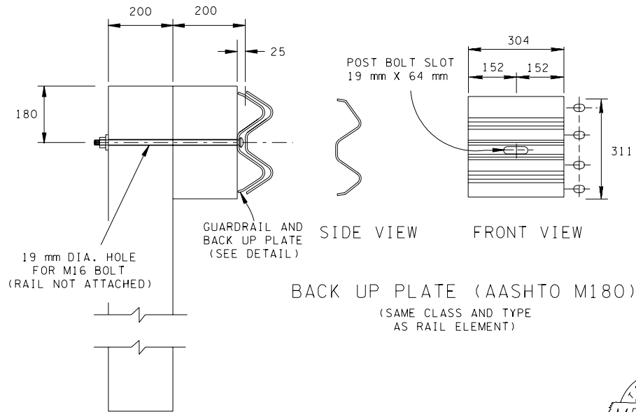
GUARDRAIL WITH BACK UP PLATE DETAIL
