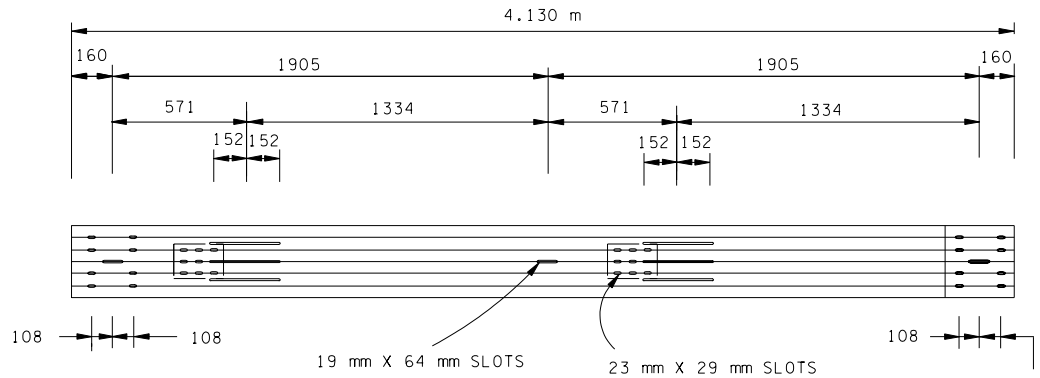
SECOND SECTION OF GUARDRAIL FOR TYPE 21 TERMINAL
