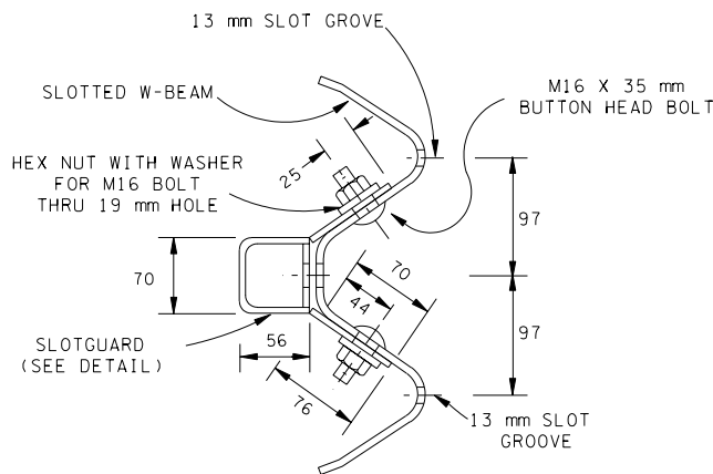
SECTION "E-E" (SEE DRAWING NO. SM-GR-26)
