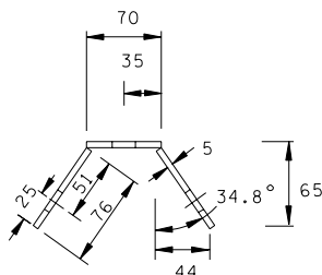
SECTION "F-F"
